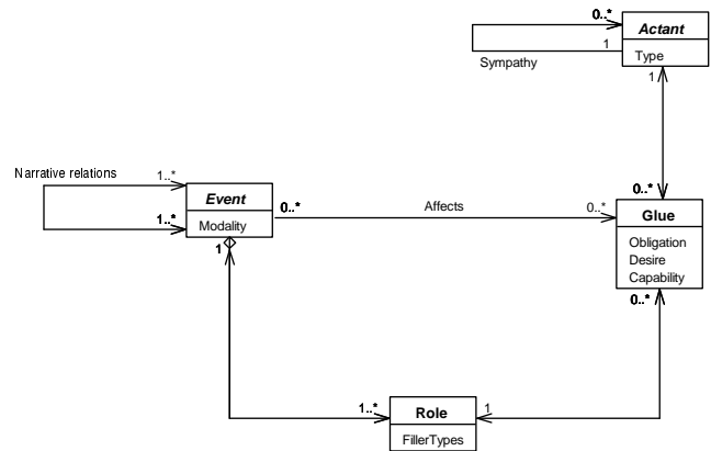
Figure 6. UML diagram of a possible narrative system.
